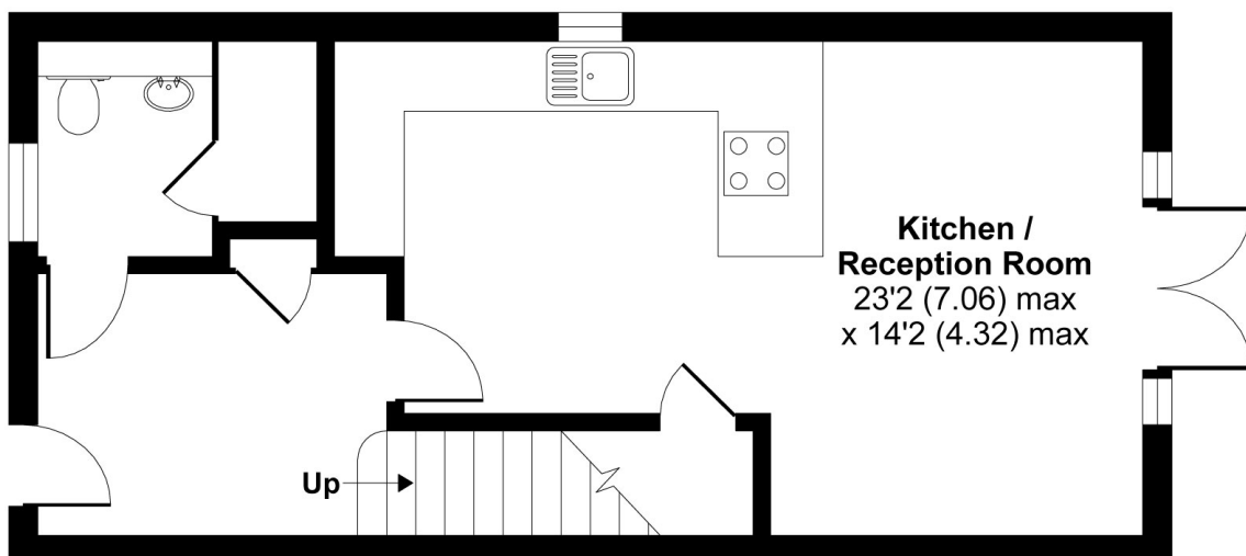
GROUND FLOOR
